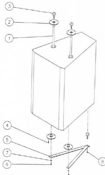
Figure 3—Exploded view of T52+ and HST2 parts
