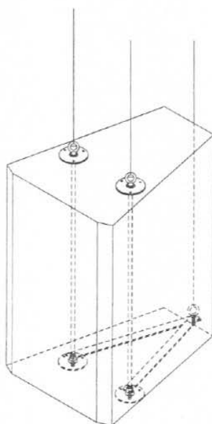
Figure 1—Suspension of T52+
